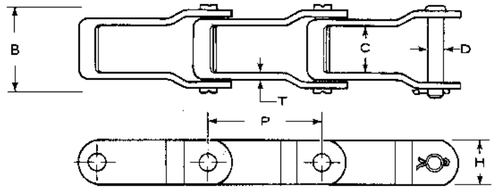
Dimension Diagram for Steel Pintle Chain
